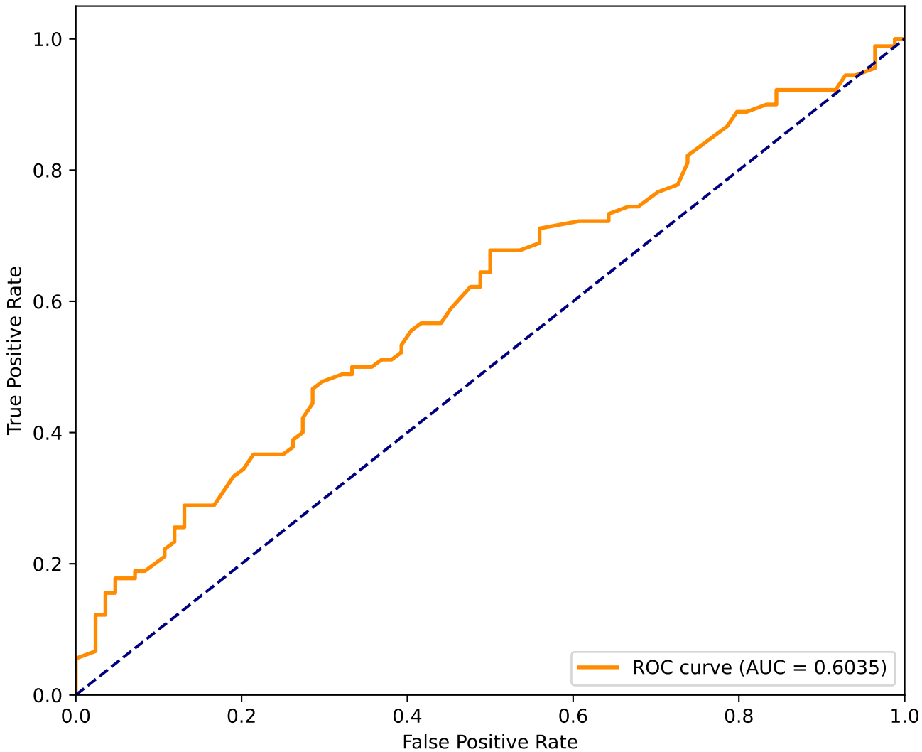
ROC Curve - ExtraTrees
